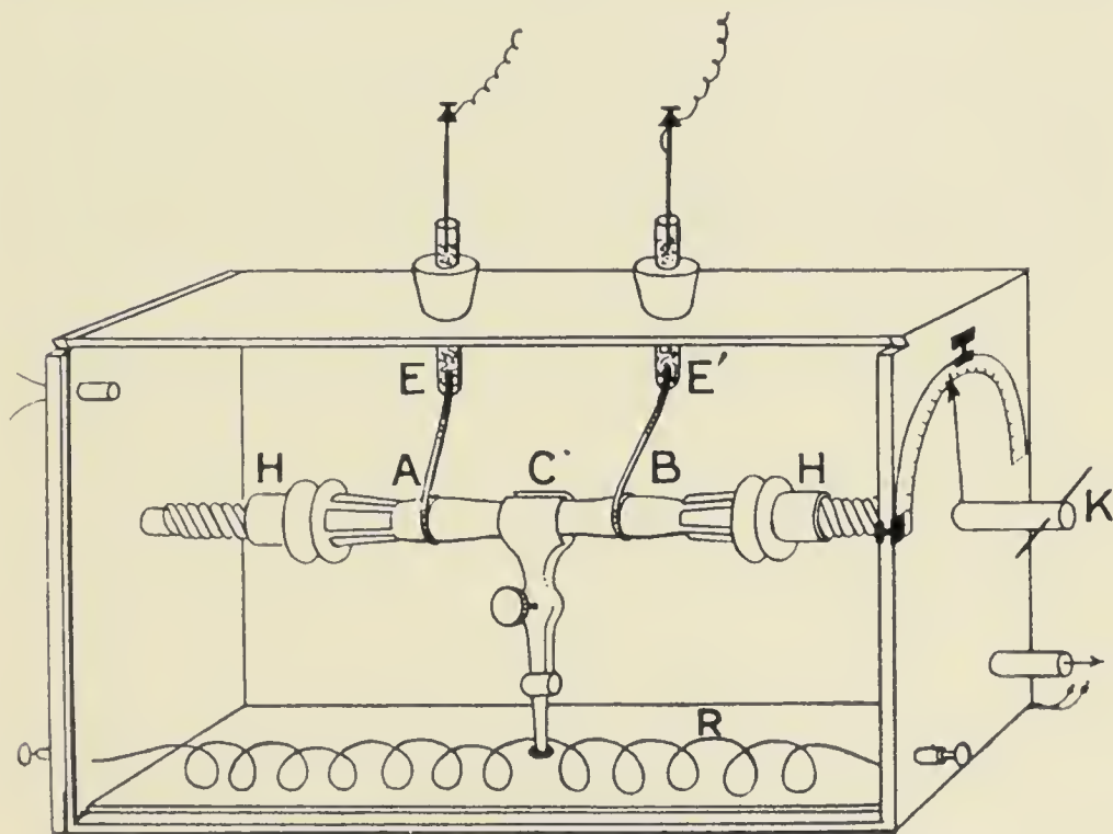
FIG. 99. The Plant-Chamber.
